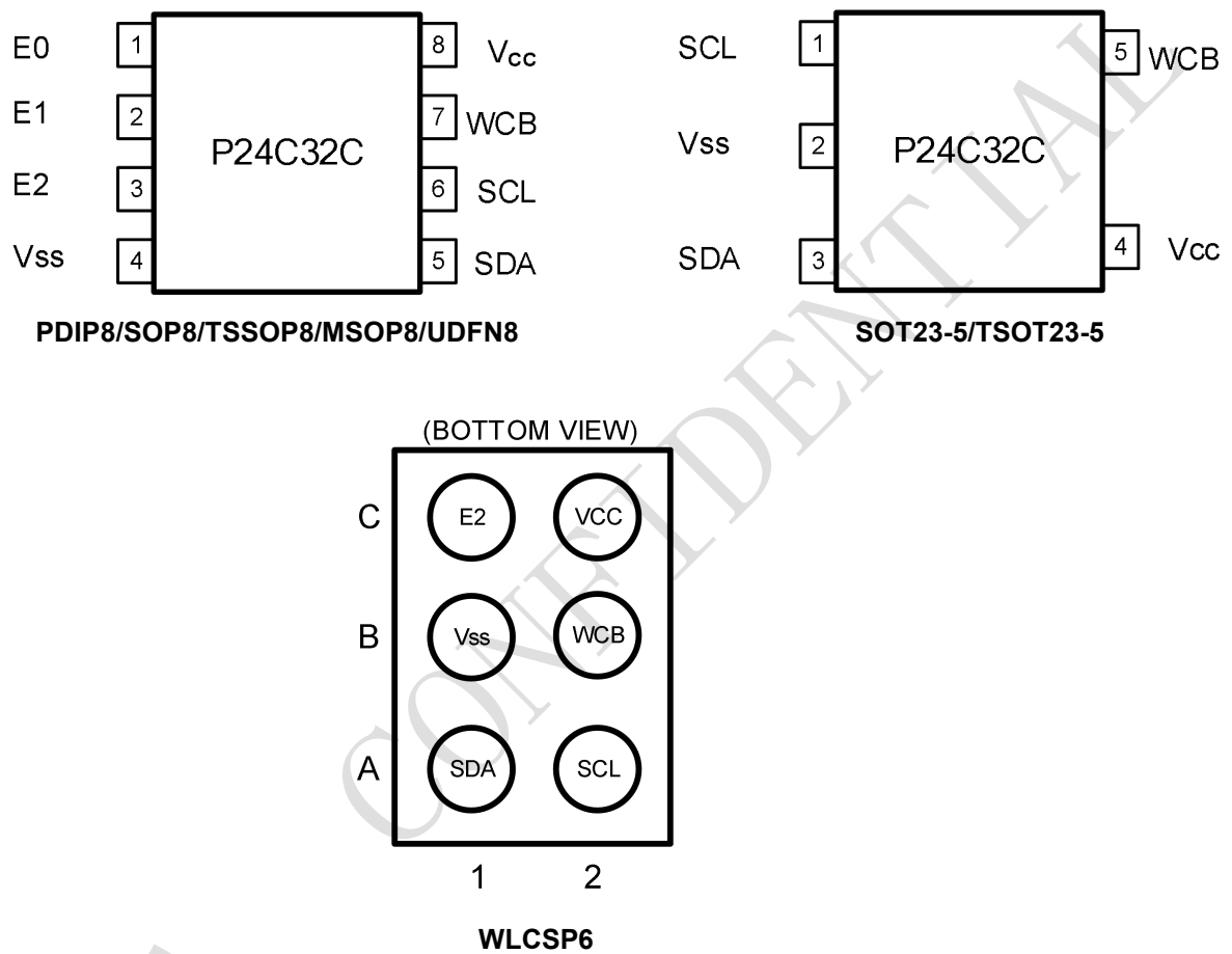
Figure 1-1 Pin Configuration
